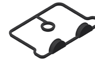
P008000005741 93536053000 HEAD COVER GASKET / JUNTA TAPA CULATA
